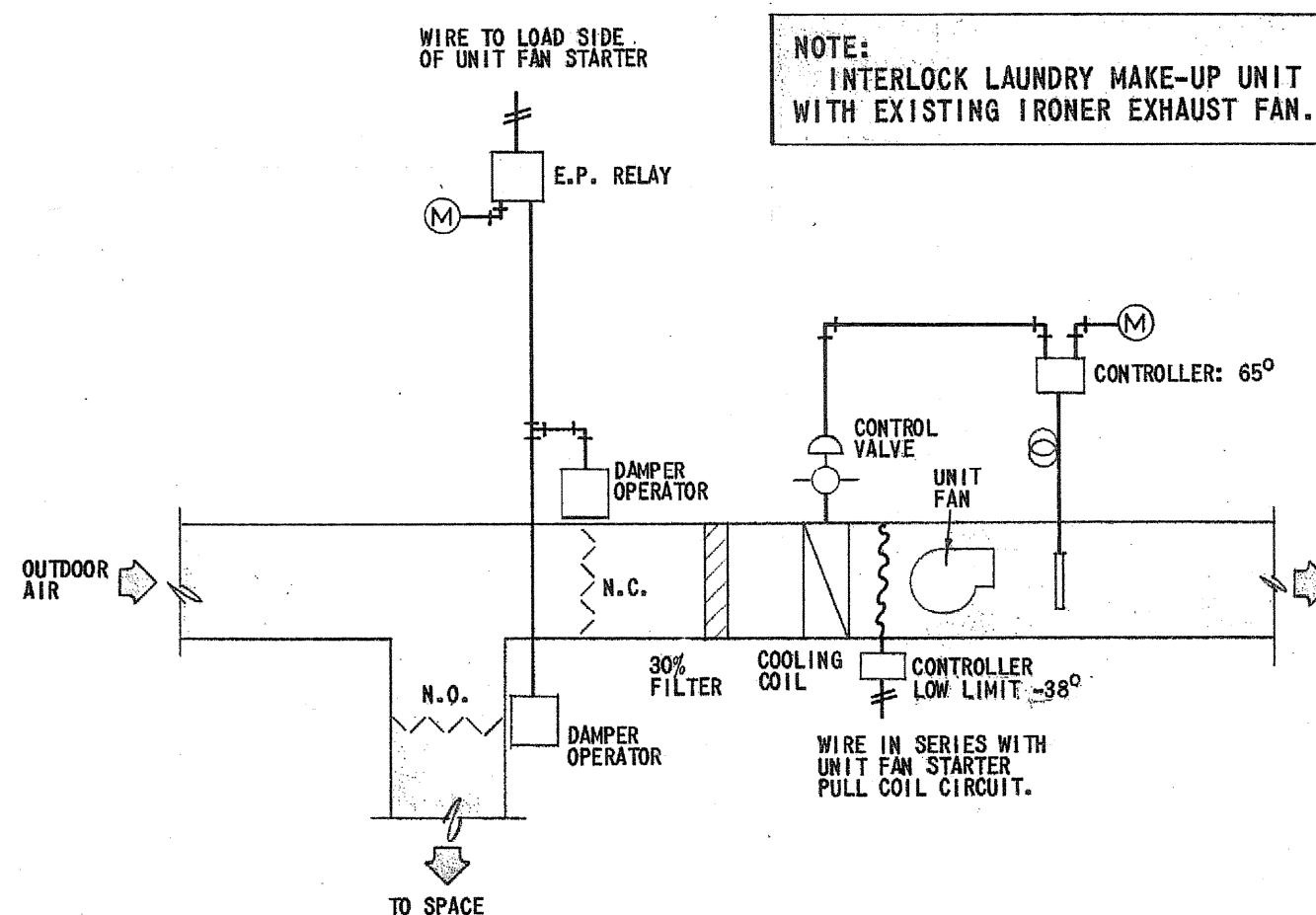
LAUNDRY MAKE-UP UNIT CONTROLS Scale
