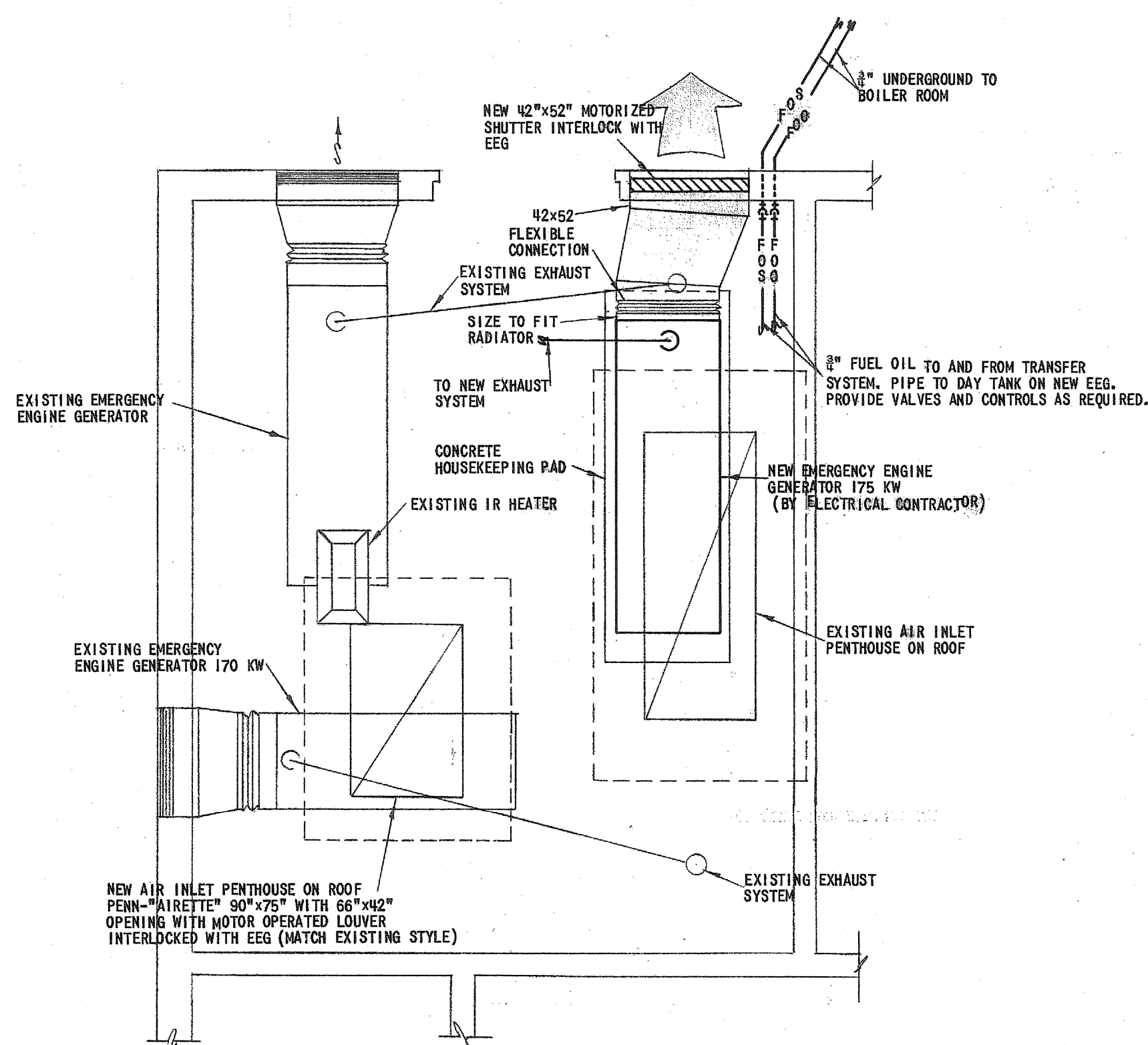
ENGINE GENERATOR ROOM PARTIAL PLAN Scale 1/4" = 1'-0"
